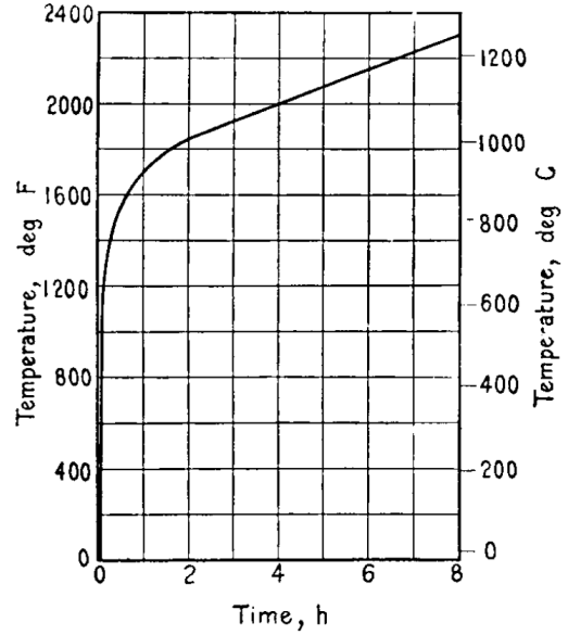
FIG. 1 Time-Temperature Curve
